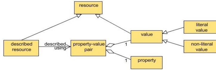
الشكل (3) : Class diagram for DCMI resource model [18]
