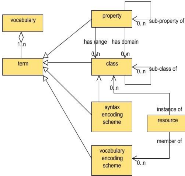
الشكل (4) : Class diagram for DCMI vocabulary model [18]
